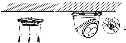
Figure 2-5 Fix the camera to the ceiling
