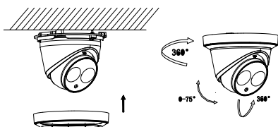
Figure 2-6 Install the trim ring
