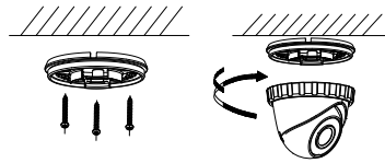
Figure 2-7 Fix the Mounting Base and Camera
