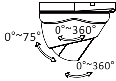
Figure 2-3 3-axis Adjustment
