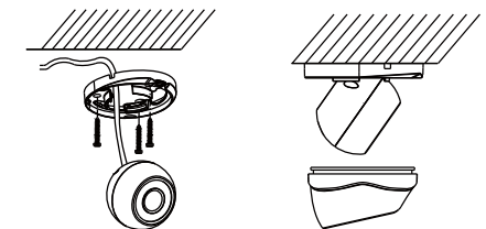
Figure 2-2 Fix the Mounting Base and the Camera
