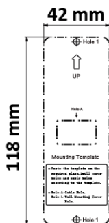
Figure 2-2 Mounting Template
